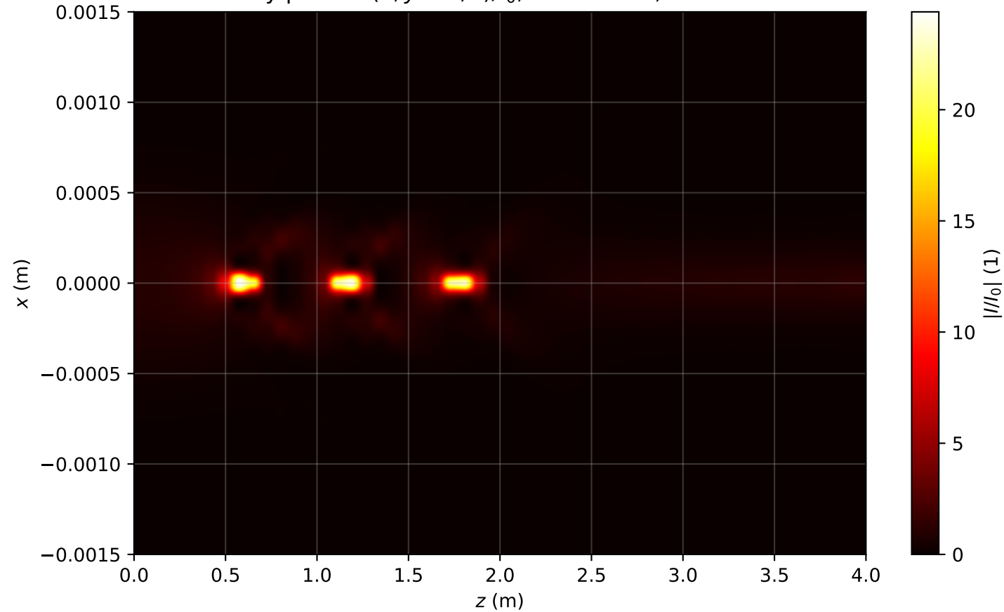
Intensity profile I(x, y = 0, z)/I_0 , P_{in}=4.5P_{cr} , artificial time
